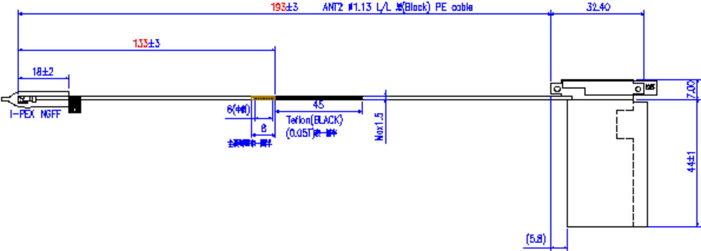
Tx2 (or Rx2) Antenna Dimensioned Drawing:
