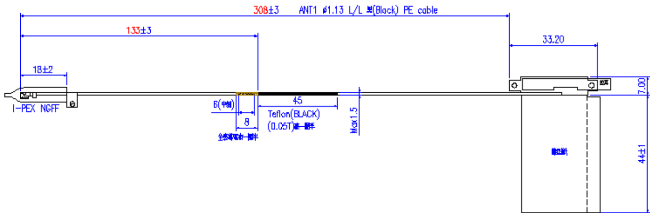
Tx1 Antenna Dimensioned Drawing:
