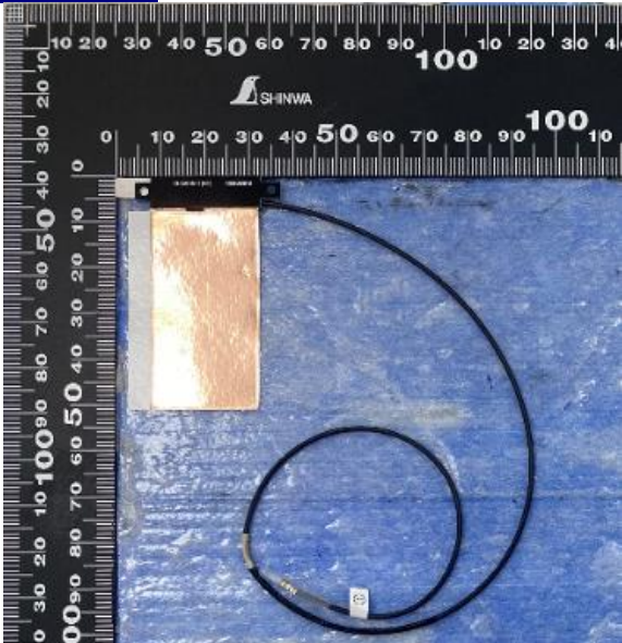
Tx1 Antenna Photo:
