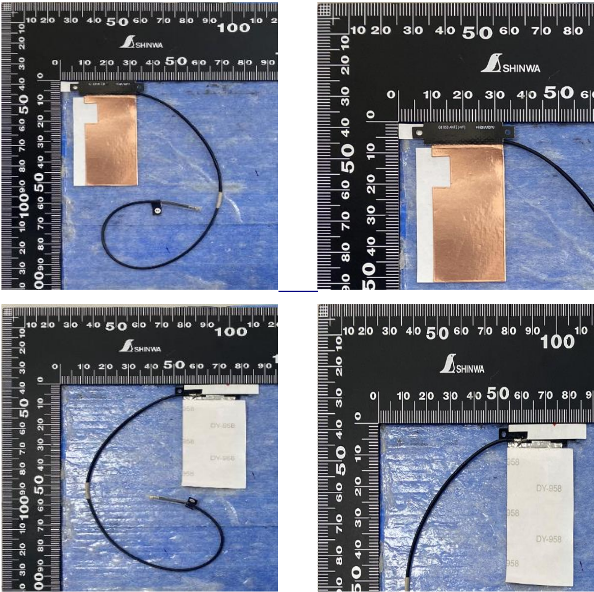
Tx2 (or Rx2) Antenna Photo:
