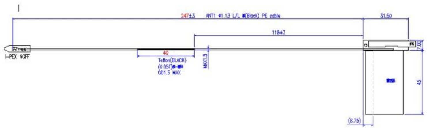
Tx1(or Rx1) Antenna Dimensioned Drawing:
