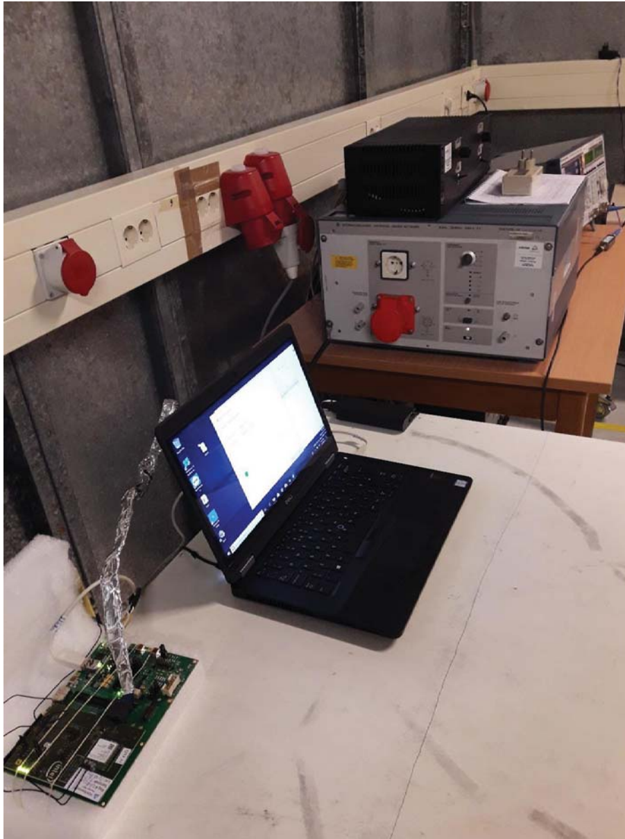
Photo 5: Photograph conducted emissions 0.15-30 MHz
