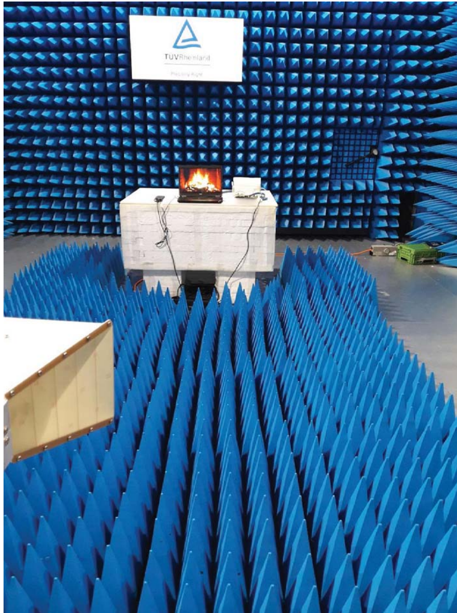
Photo 2: Photograph radiated emissions 1 – 6 GHz
