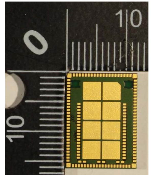
Back Side
