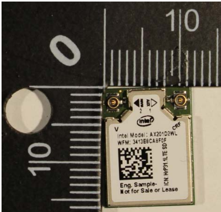
Front Side
