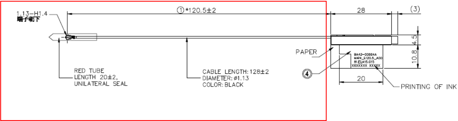
Tx1(or Rx1) Antenna Dimensioned Drawing:
