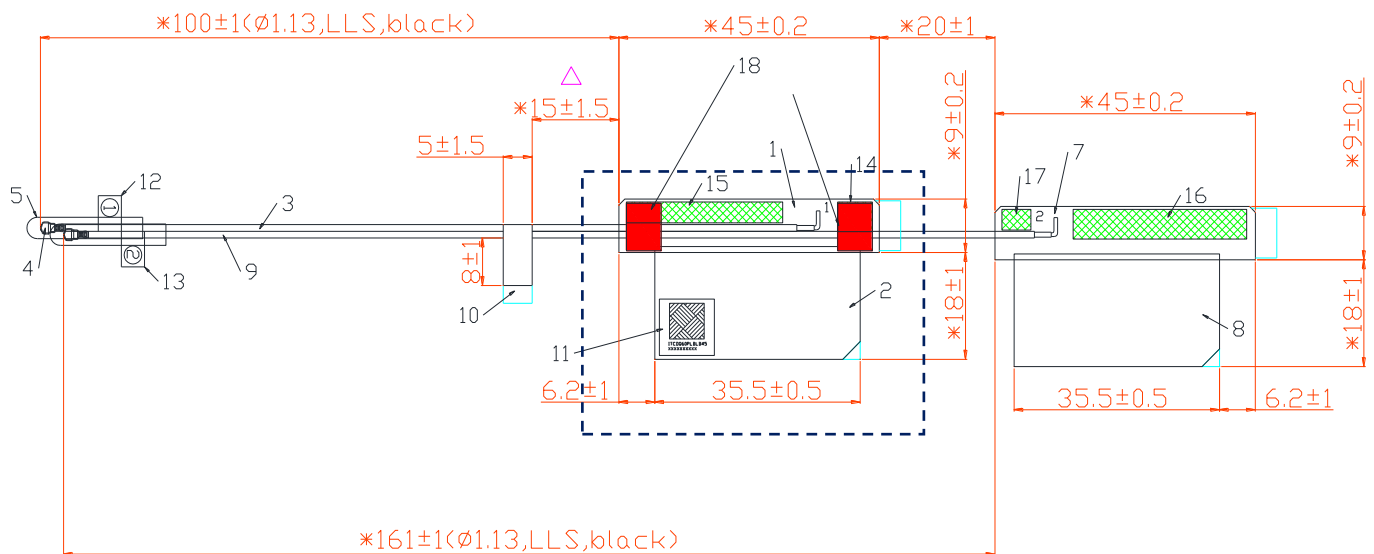
Tx1 Antenna Dimensioned Drawing:
