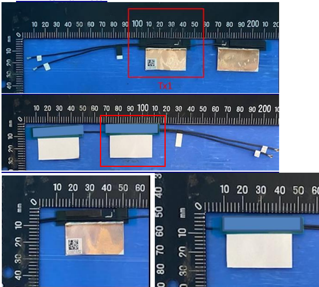
Tx1 Antenna Photo:
