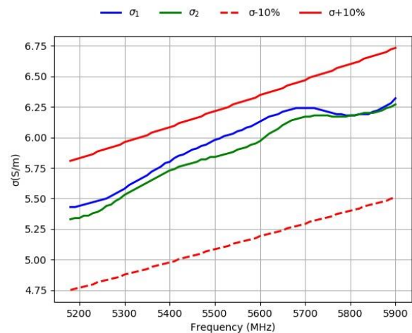
Conductivity
