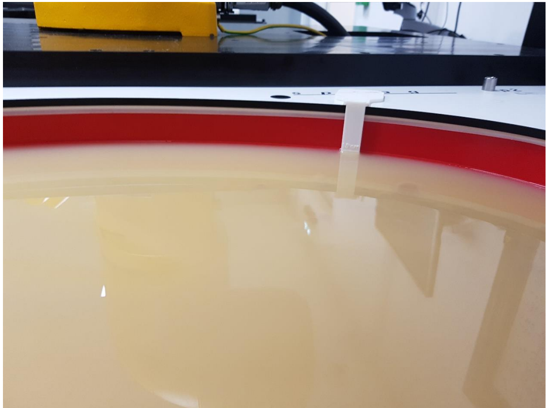
ELI phantom Body liquid SAR Dasy SPEAG MBBL600-6000V6 Batch - 160630-01
