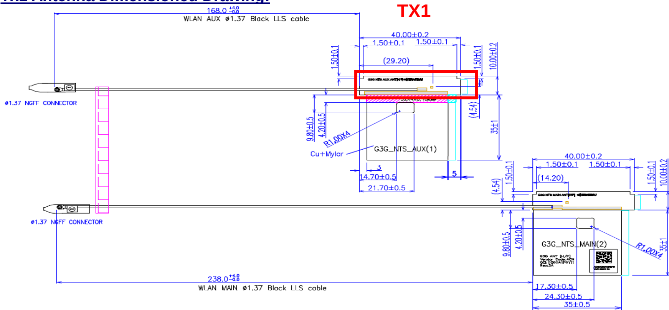
Tx1 Antenna Dimensioned Drawing:
