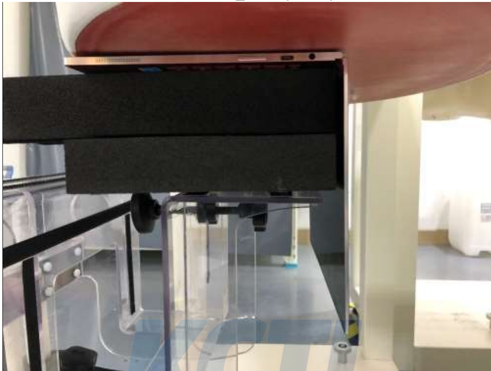
Notebook_Rear (0 mm)
