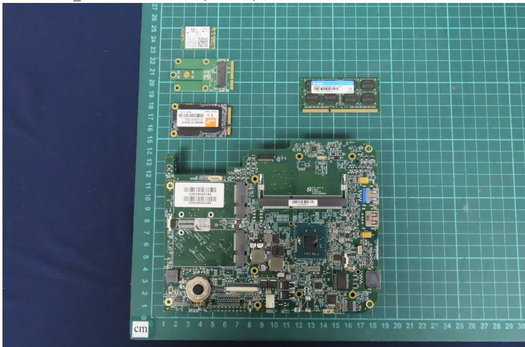
(68) EUT Photo_M/N: 3571-0100-5x (TMVCI)
