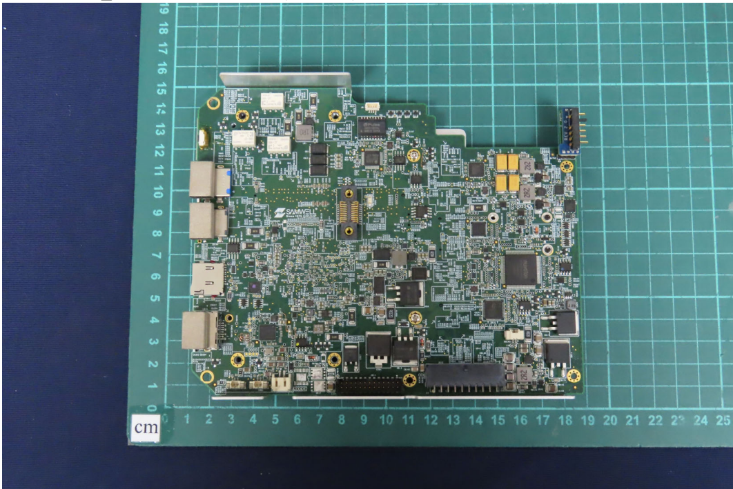
(64) EUT Photo_M/N: 3571-0100-5x (TMVCI)
