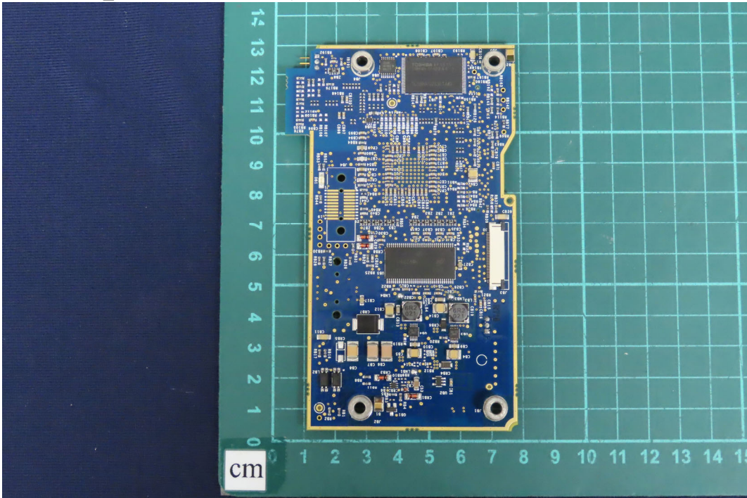
(63) EUT Photo_M/N: 3571-0100-5x (TMVCI)
