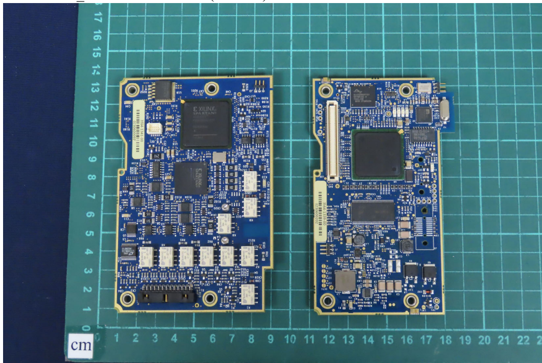
(59) EUT Photo_M/N: 3571-0100-5x (TMVCI)
