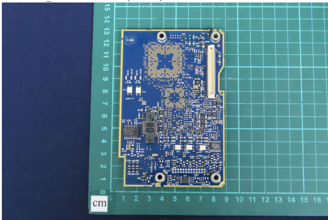
(61) EUT Photo_M/N: 3571-0100-5x (TMVCI)
