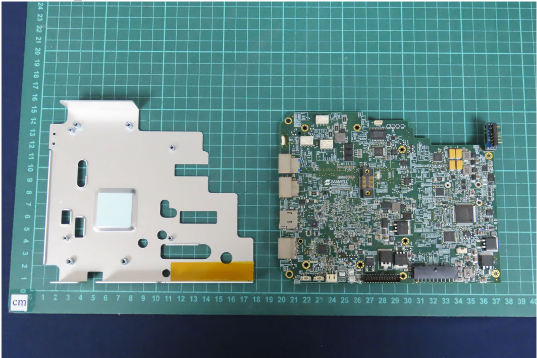
(65) EUT Photo_M/N: 3571-0100-5x (TMVCI)
