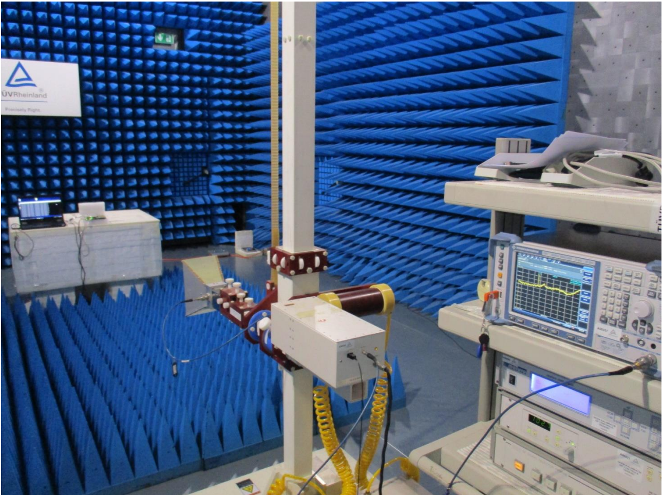
Photo 3: Photograph radiated emissions 6 – 18 GHz
