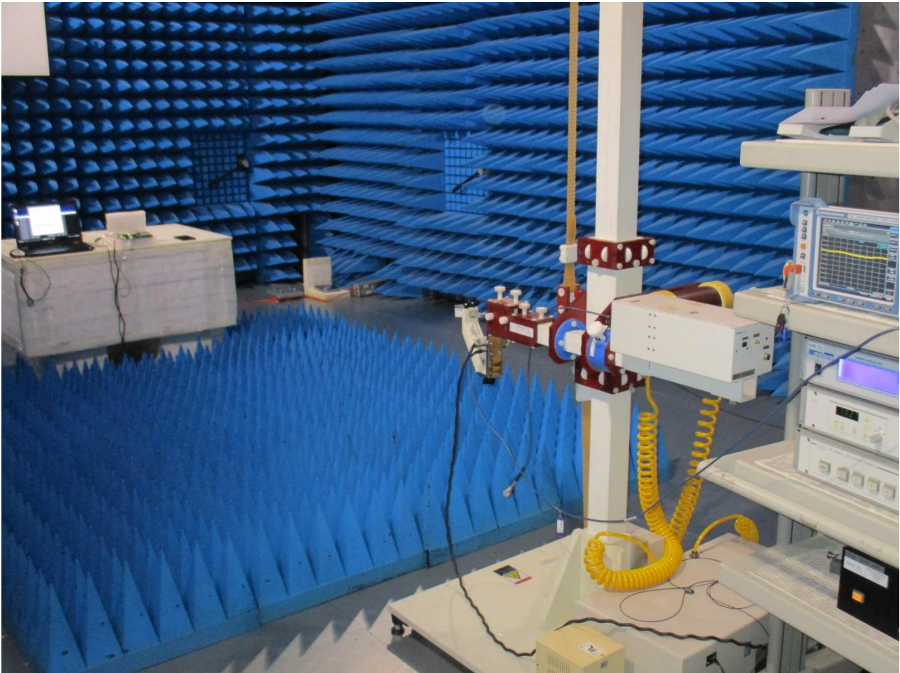
Photo 4: Photograph radiated emissions 18 – 30 GHz
