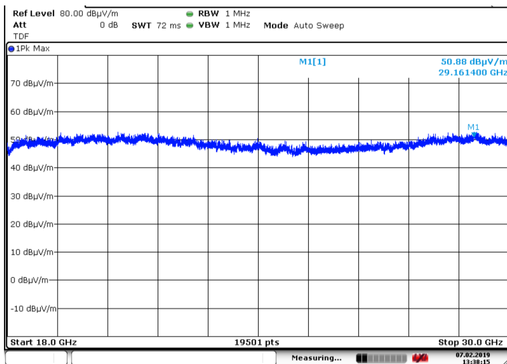
Plot 8: Pre-scan plot with peak detector. Radiated emissions from 18 GHz – 30 GHz, 5 GHz WIFI and BT mode
