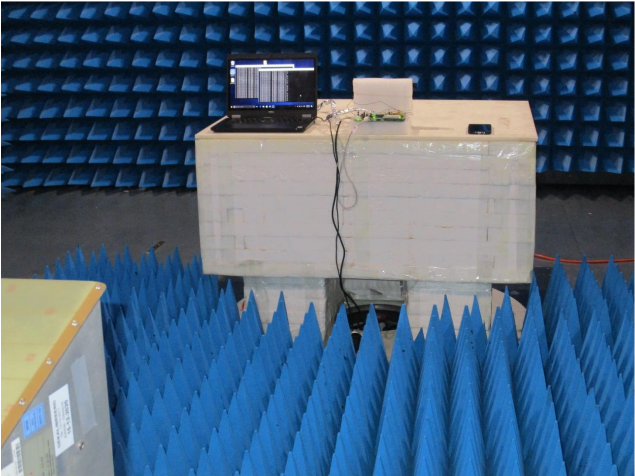
Photo 2: Photograph radiated emissions 1 – 6 GHz
