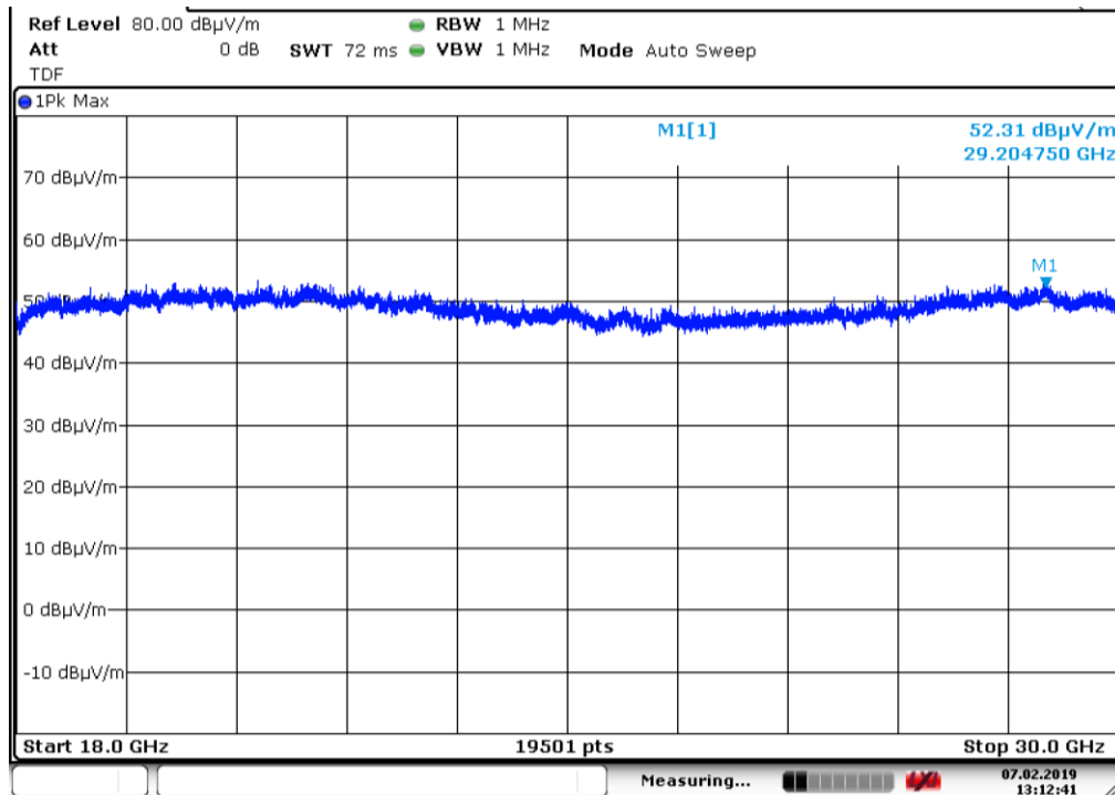
Plot 7: Pre-scan plot with peak detector. Radiated emissions from 18 GHz - 30 GHz, 2.4 GHz WIFI mode
