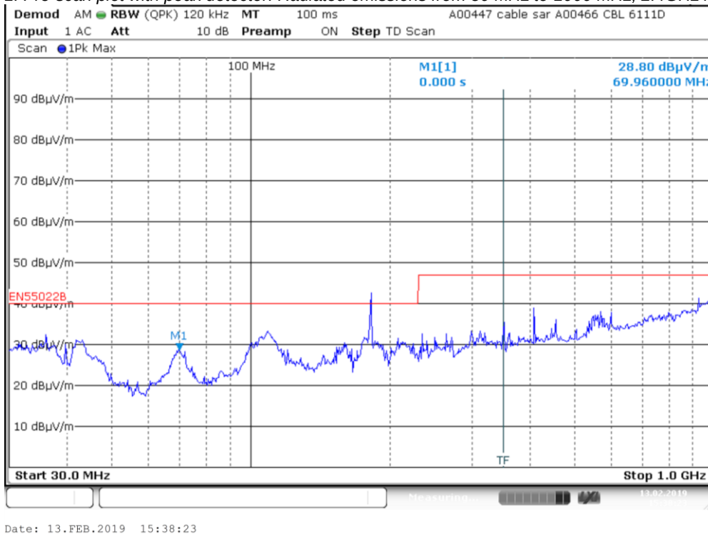
Plot 2: Pre-scan plot with peak detector. Radiated emissions from 30 MHz to 1000 MHz, 5GHz and BT mode.
