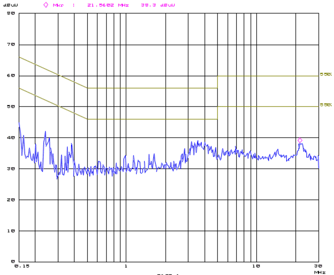
Plot 10: Pre-scan plot with peak detector. Conducted emissions from 0.15 - 30 MHz, 5 GHz WIFI and BT mode
