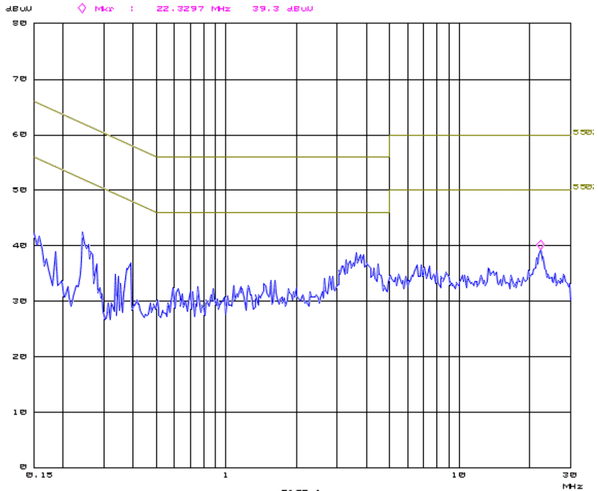
Plot 9: Pre-scan plot with peak detector. Conducted emissions from 0.15 - 30 MHz, 2.4 GHz WIFI mode
