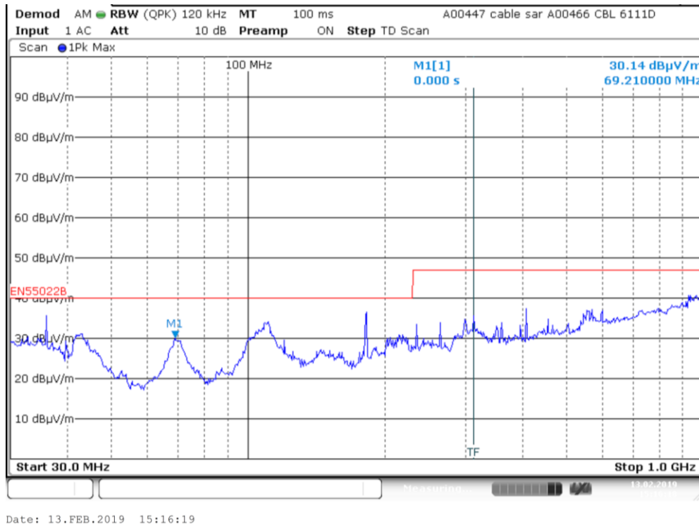
Plot 1: Pre-scan plot with peak detector. Radiated emissions from 30 MHz to 1000 MHz, 2.4GHz mode.
