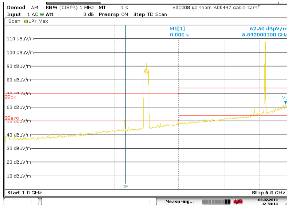
Plot 3: Pre-scan plot with peak detector. Radiated emissions from 1 GHz – 6 GHz, 2.4 GHz mode
