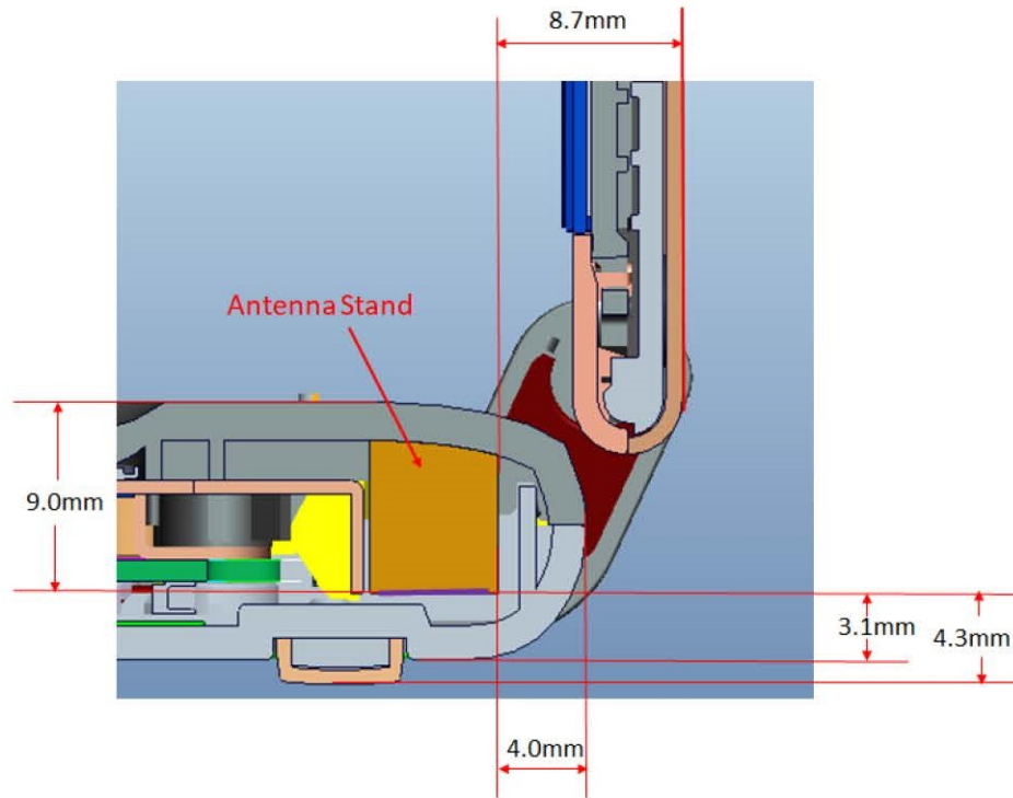
Panel open 90°
