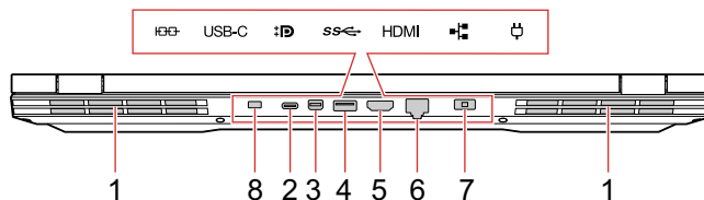
Figure 8. Legion Y540-17 series - rear view
