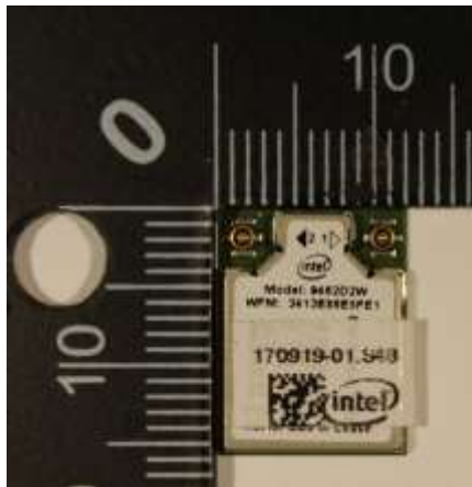
Socket Front
