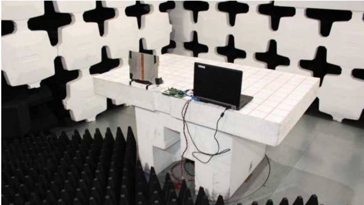
EUT arrangement
