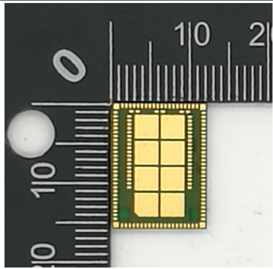
Socket Back
