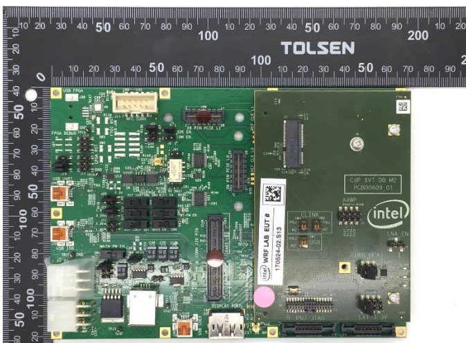
Extender board
