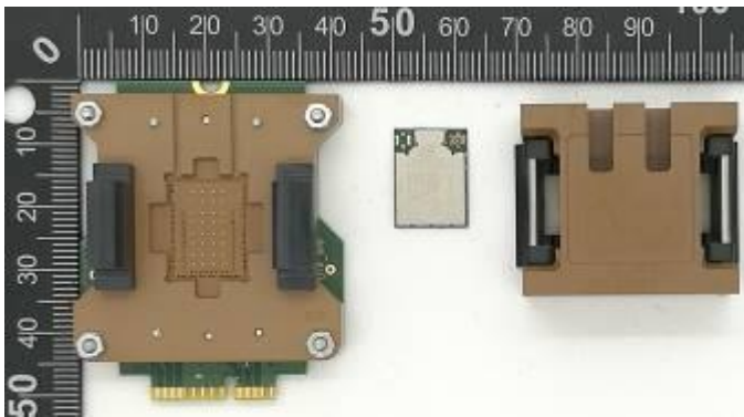
Extender board
