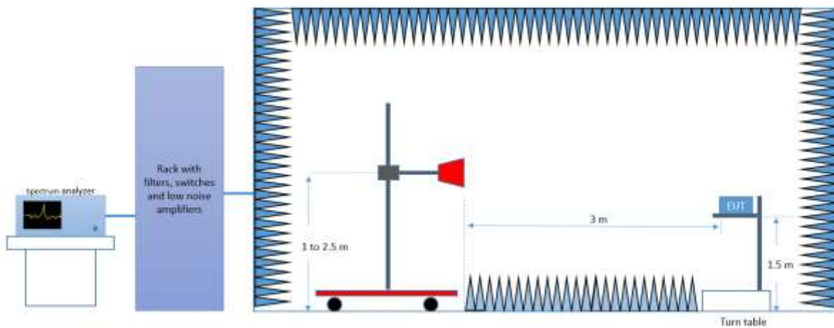
Radiated Setup 18 GHz - 25 GHz
