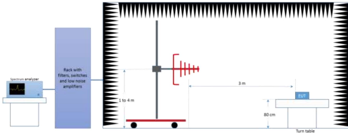
Radiated Setup 1 GHz - 18 GHz
