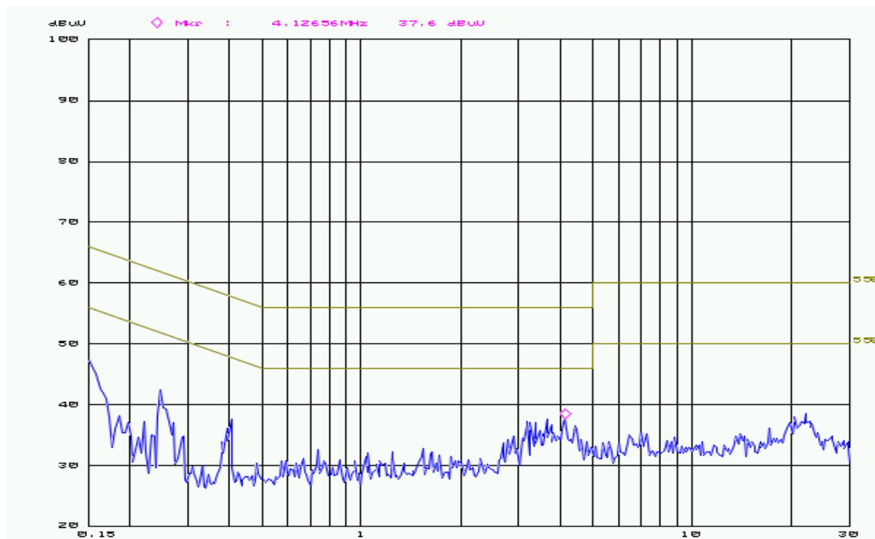
Plot 2. Conducted emission 9260NGW, max levels recorded
