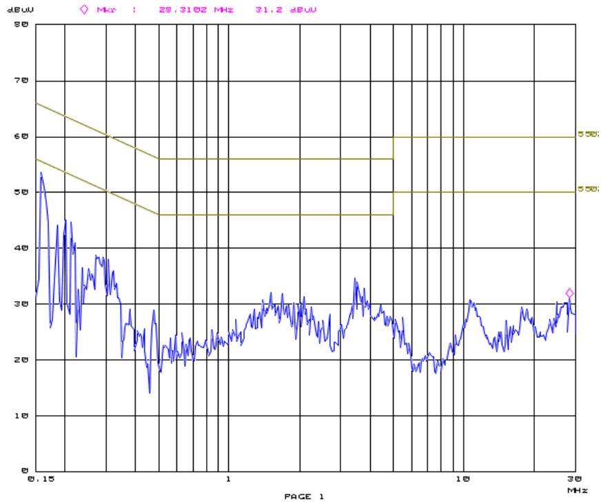
Plot 2: Conducted emission
