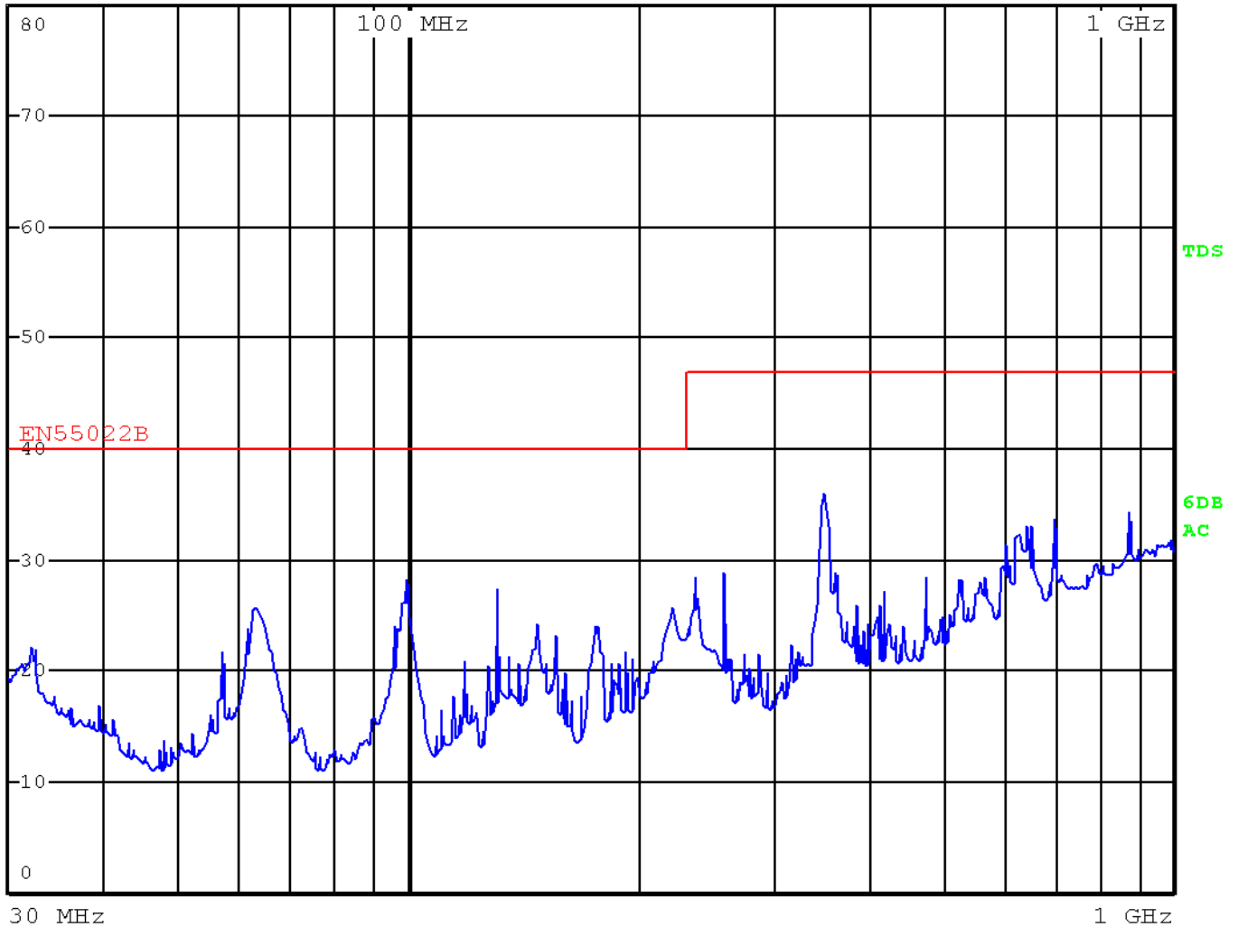
Plot 1: Radiated emissions of the EUT using wifi 2.4Ghz + Bluetooth
