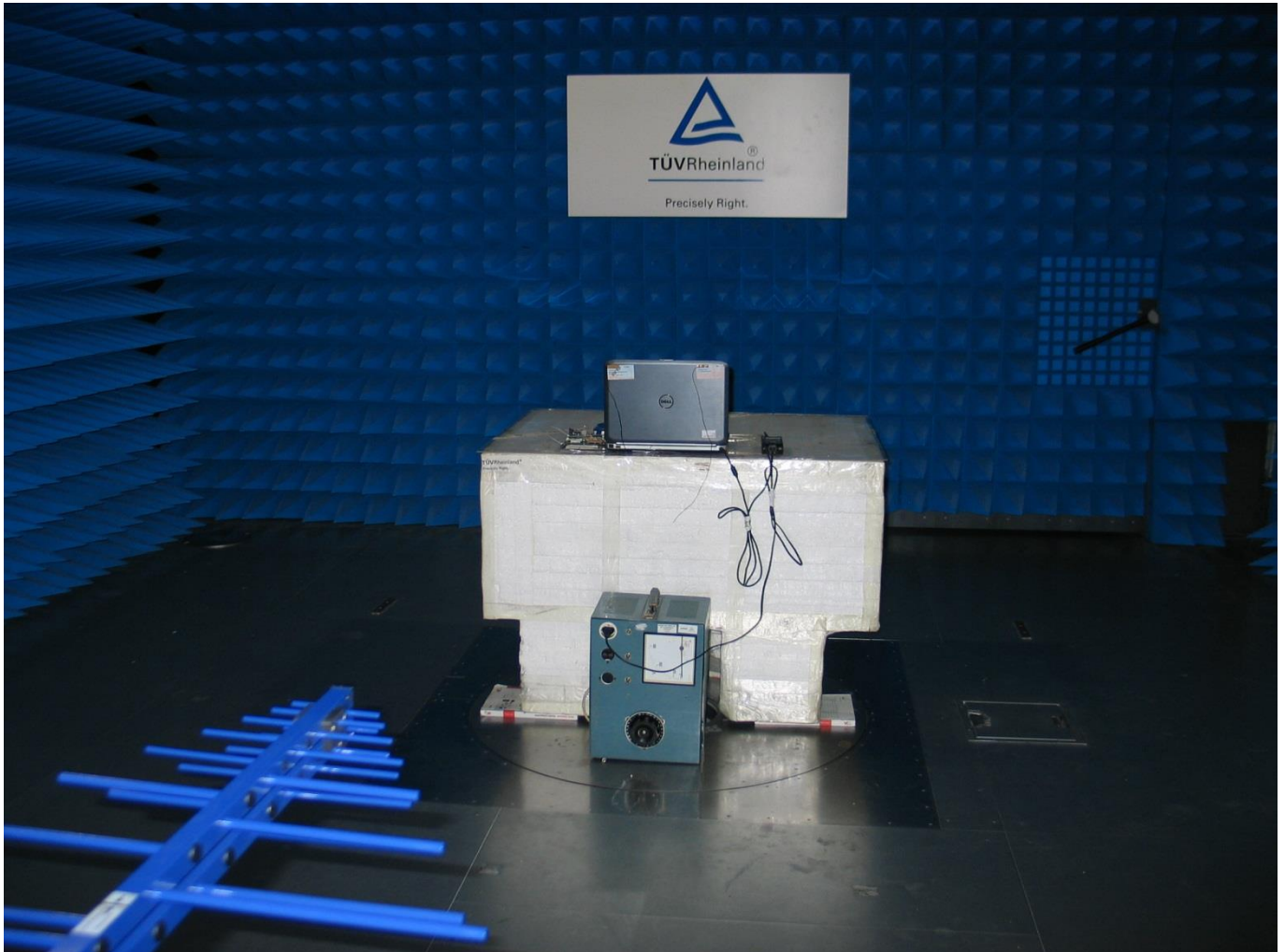
Photo 1. Radiated emission
