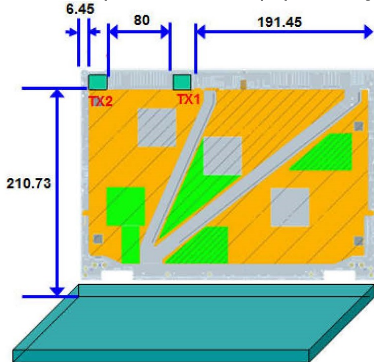
Location and Separation Distances Laptop Mode Diagrams
