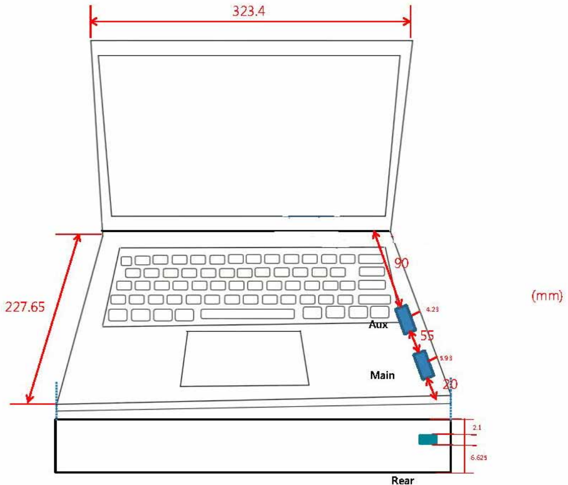
<The Distance information of Antenna to Edges of Notebook>
