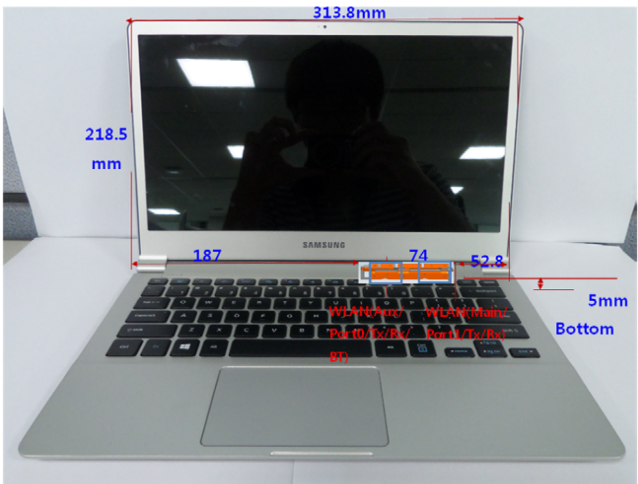
<The Distance information of Antenna to Edges of Notebook>
