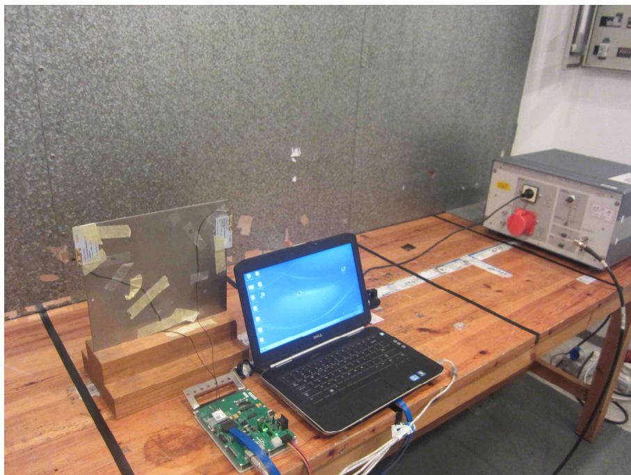
Fig. 7. Test set-up for conducted measurements
