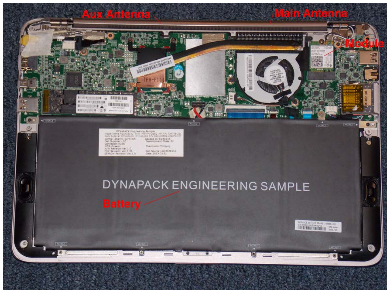
Component Locations Looking from Bottom of Device
