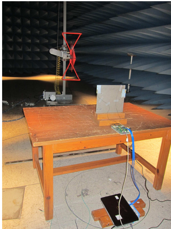
Fig. 4. Test set-up for radiated measurements above 30MHz to 1GHz
