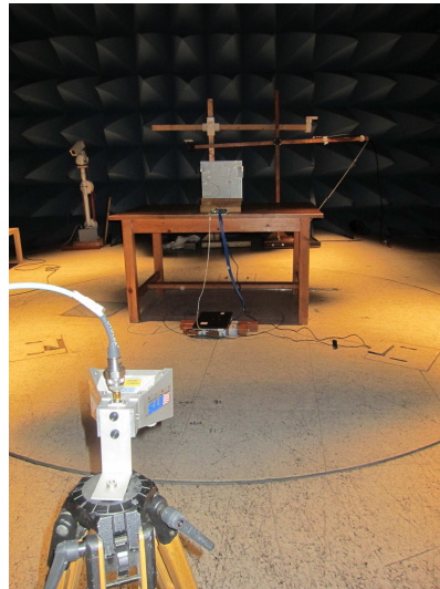
Fig. 6. Test set-up for radiated measurements above 18GHz to 40GHz
