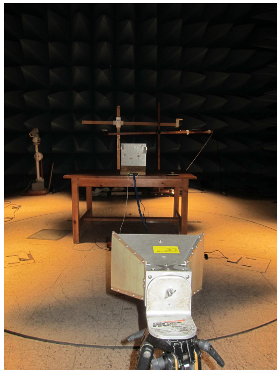
Fig. 5. Test set-up for radiated measurements above 1GHz to 18GHz
