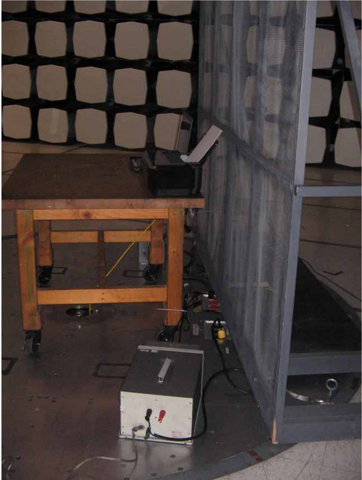
Conducted Emissions Test Configuration Photographs
