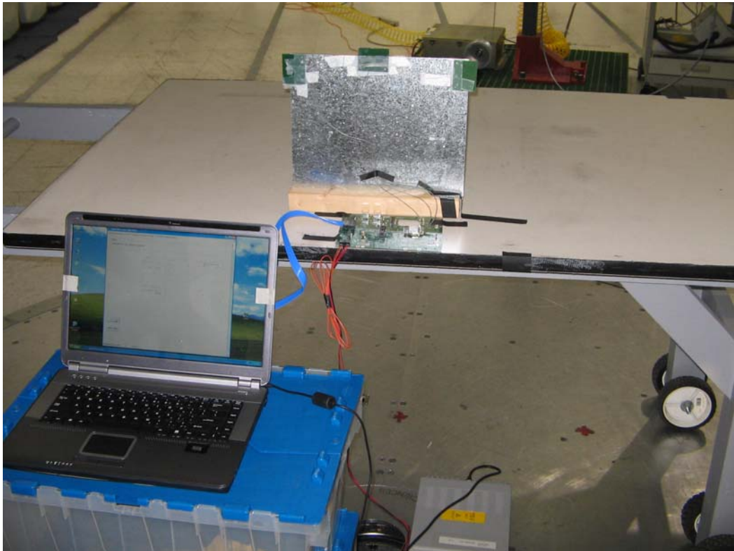
Bottom photograph shows a close-up of test fixture board (horizontal) and the three antennas mounted on the vertical dummy "laptop screen"
