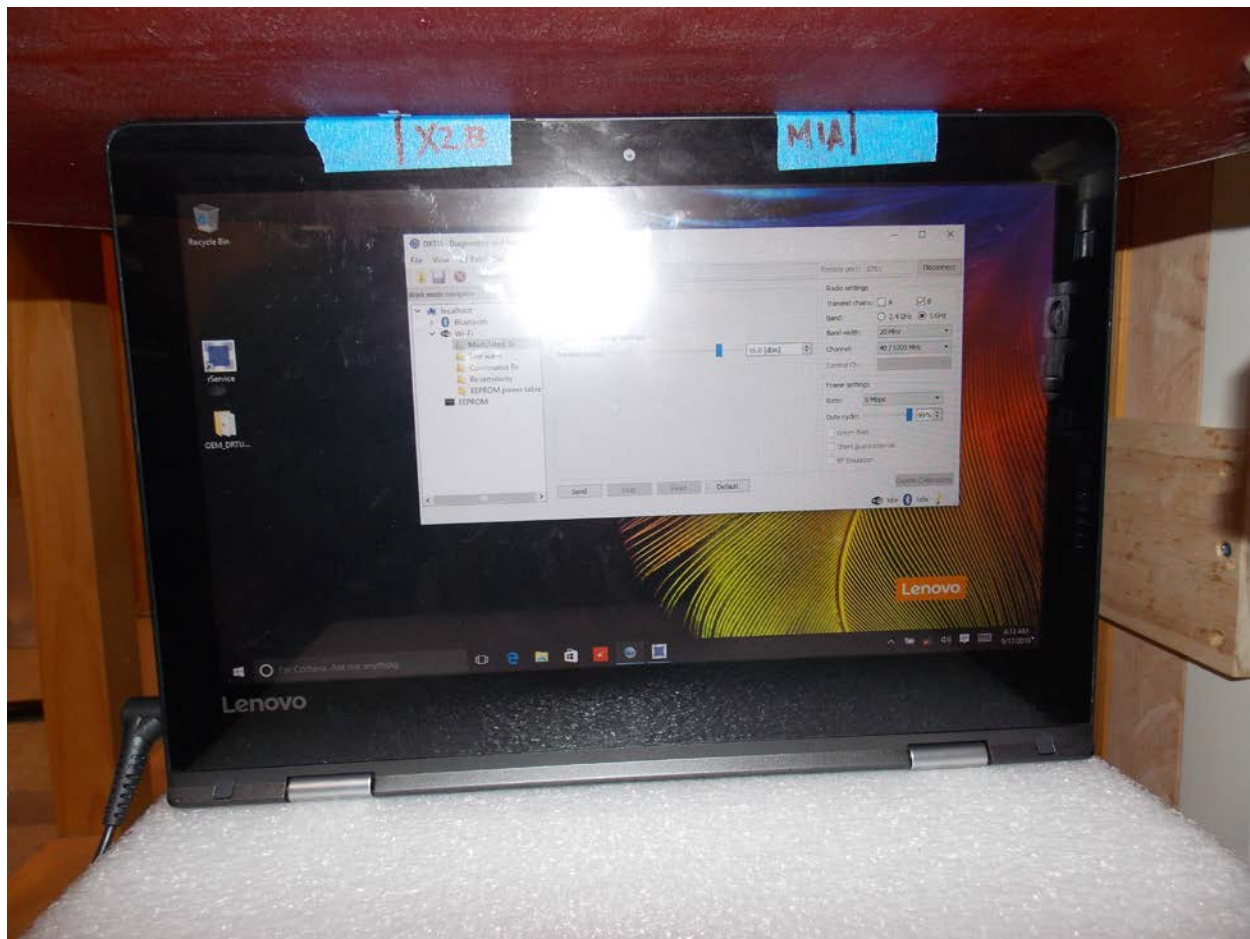
Test Position Tablet Front Edge 0 mm Gap
