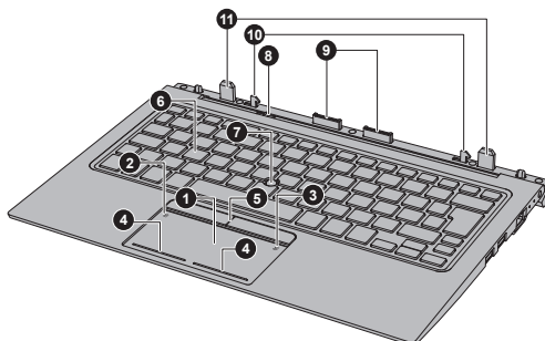
Figure 3-2 Front view of the keyboard dock
