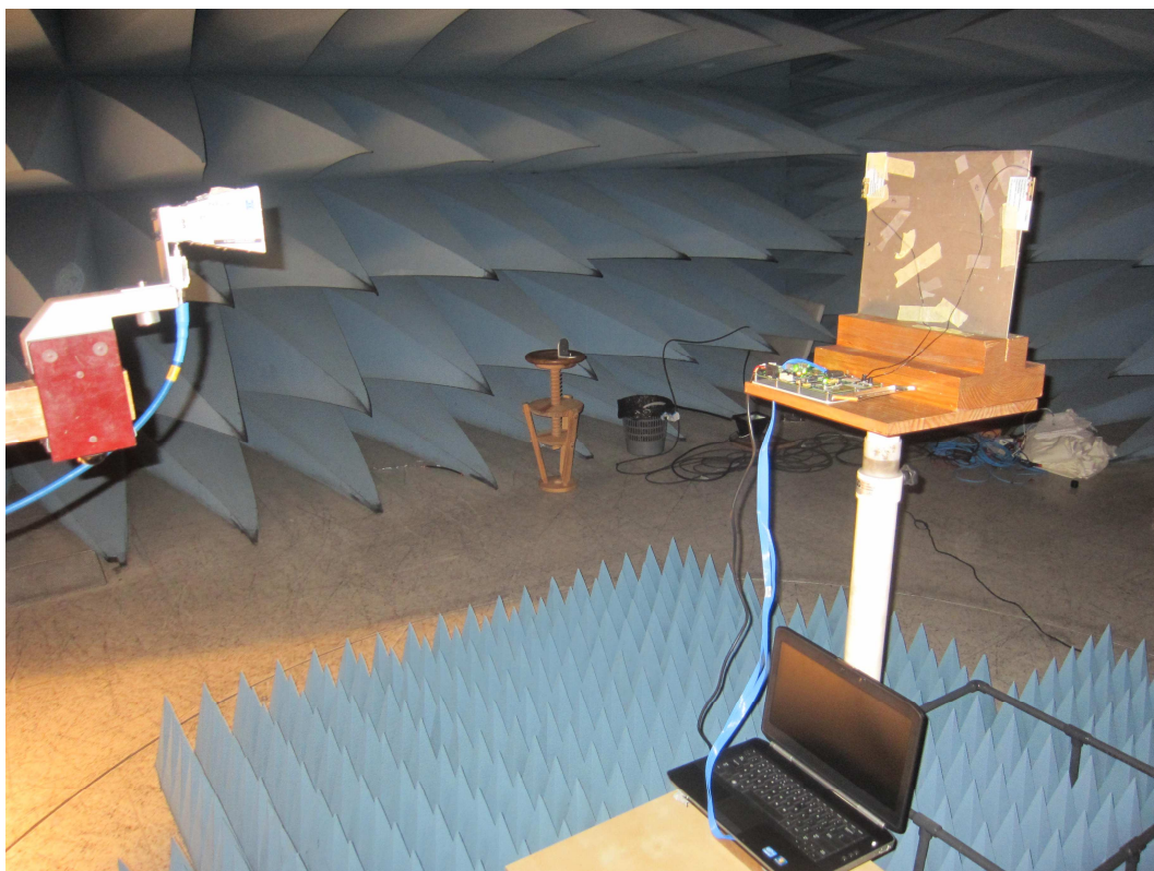
Fig. 5. Test set-up for radiated measurements above 18GHz to 40GHz
