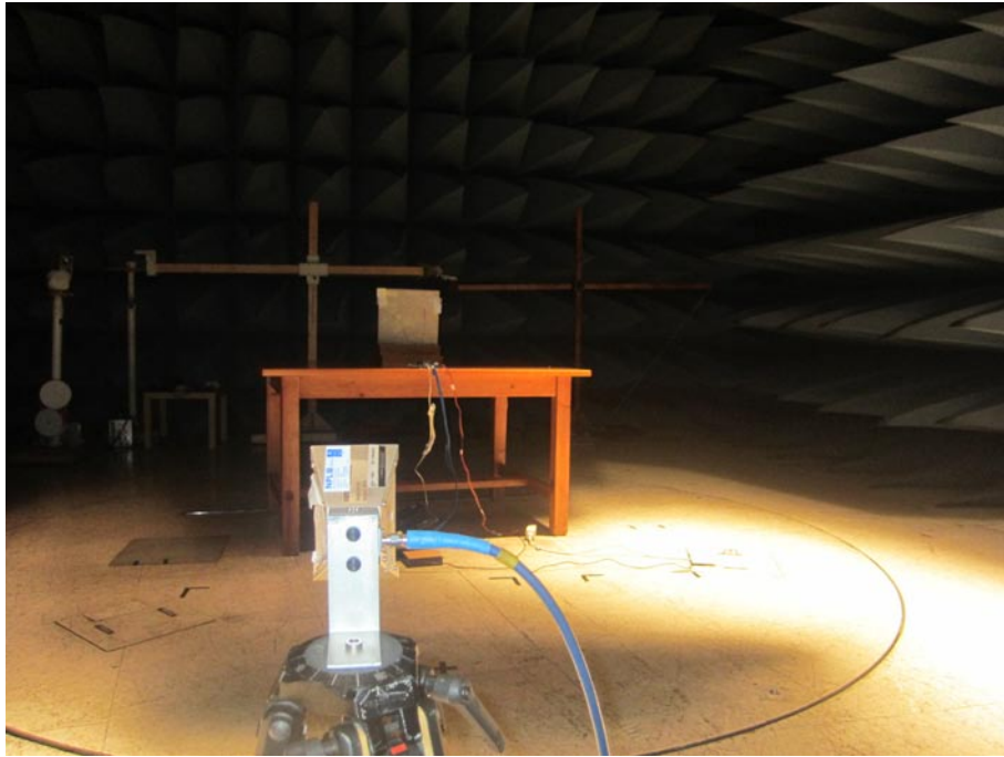
Fig. 6. Test set-up for radiated measurements above 18GHz to 26GHz
