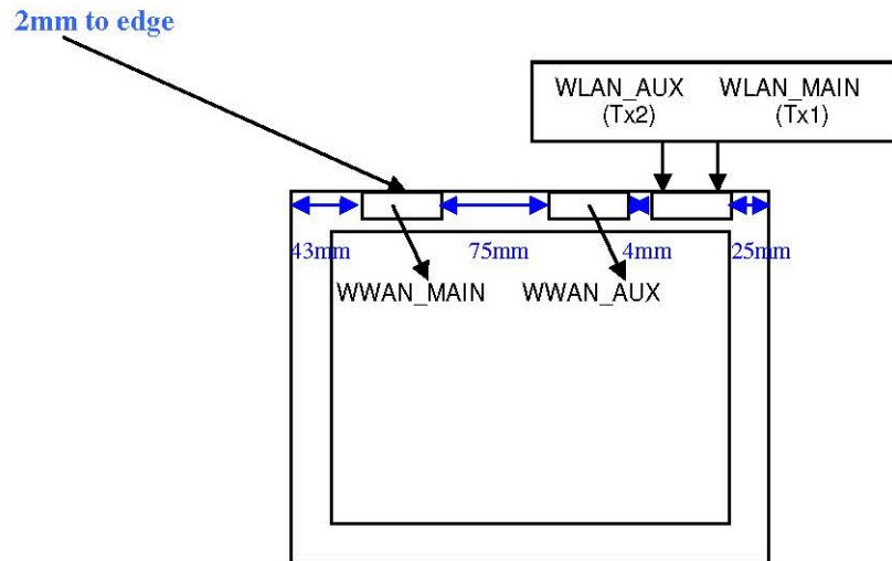
Module and Antenna Locations 13.5"
