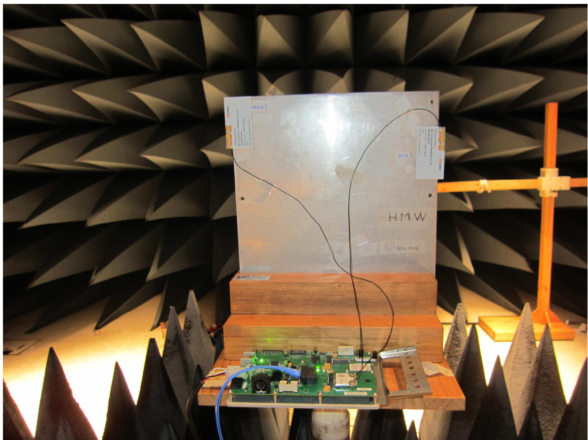
Fig. 3. Antenna frontal view
