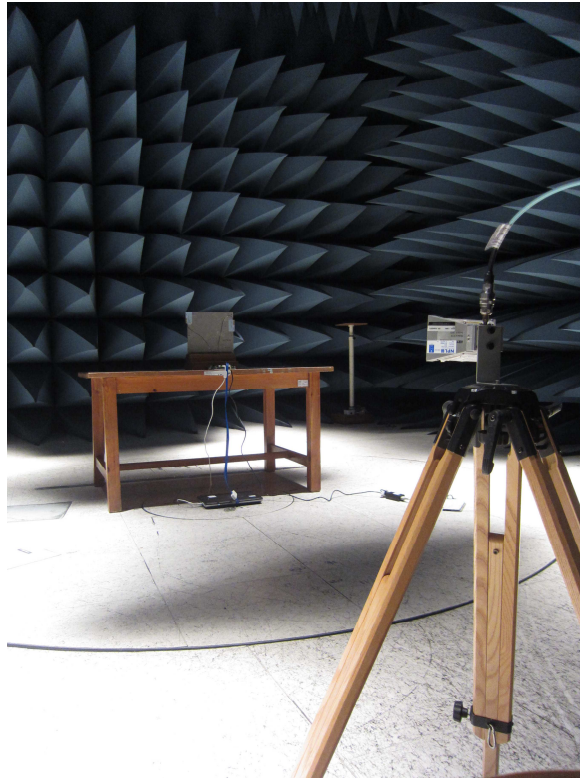
Fig. 6. Test set-up for radiated measurements above 18GHz to 26GHz
