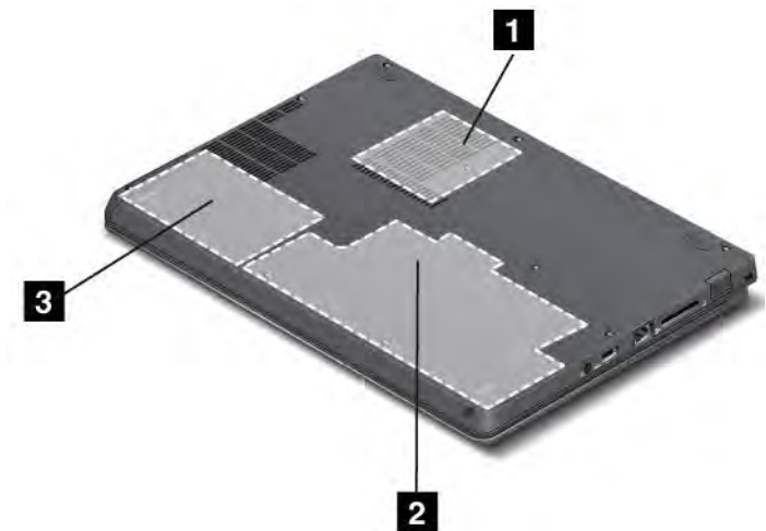
Figure 4. ThinkPad S230u bottom view
