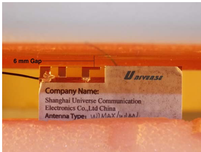
Test Position Side D 6 mm Gap
