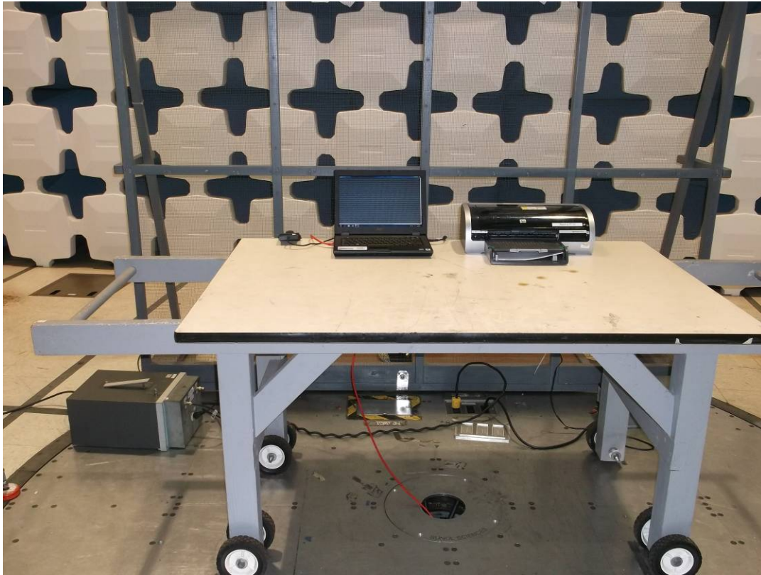
Conducted Emissions Test Configuration Photographs
