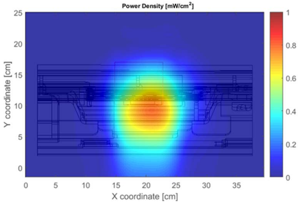
Figure 19 – Channel 2 worst case - Integrated power over 1\text{cm}^2 an platform
