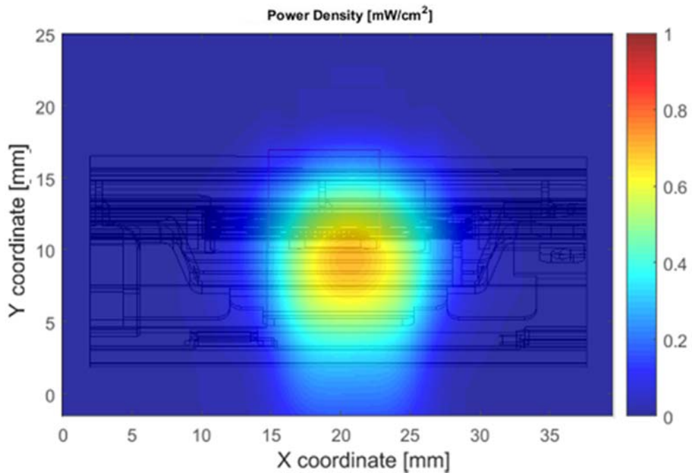
Figure 20 – Channel 3 worst case - Integrated power over 1\text{cm}^2 an platform
