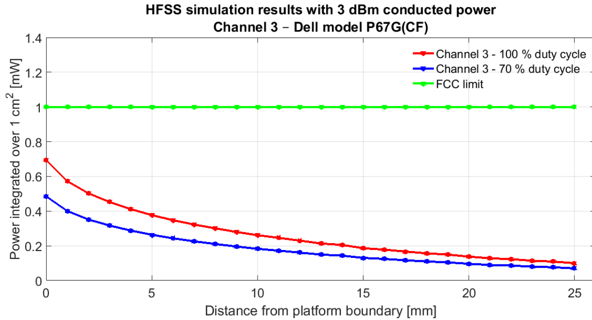
Figure 23 – HFSS Simulation results in Ch3
