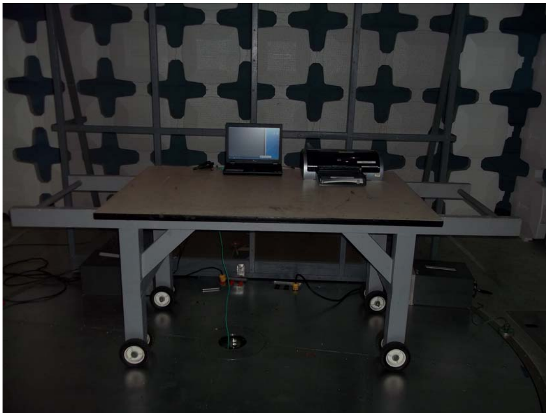
Conducted Emissions Test Configuration Photograph
