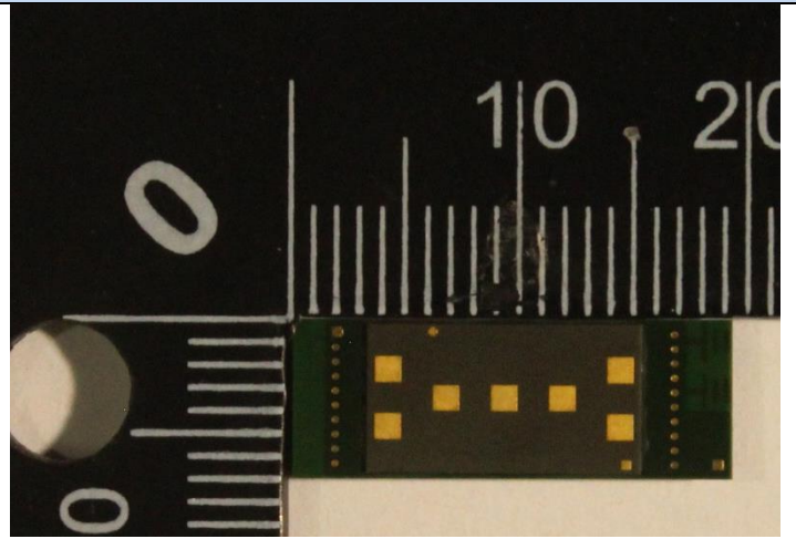
WiGig Antenna B
