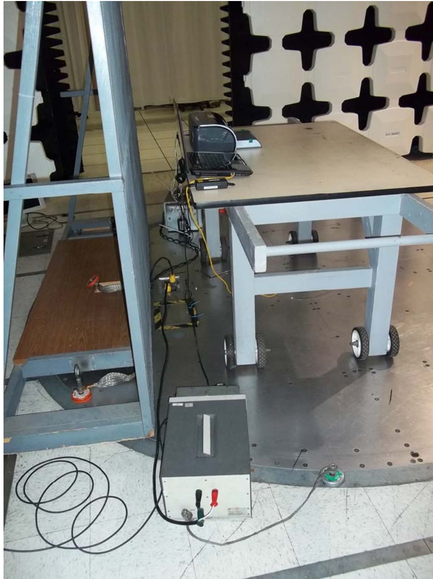
Conducted Emissions Test Configuration Photograph
