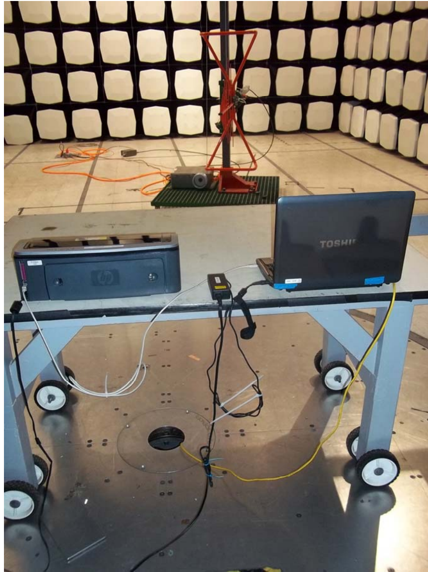
Radiated Emissions Test Configuration Photograph
