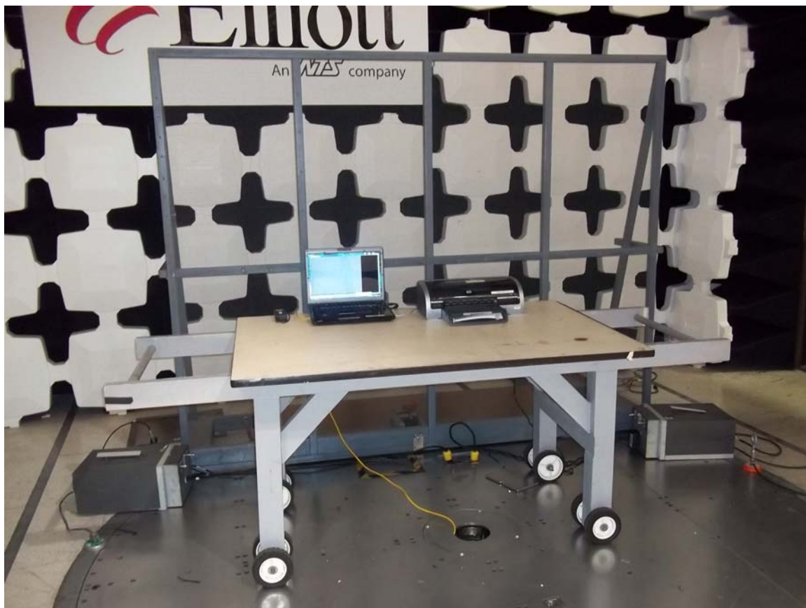
Conducted Emissions Test Configuration Photograph
