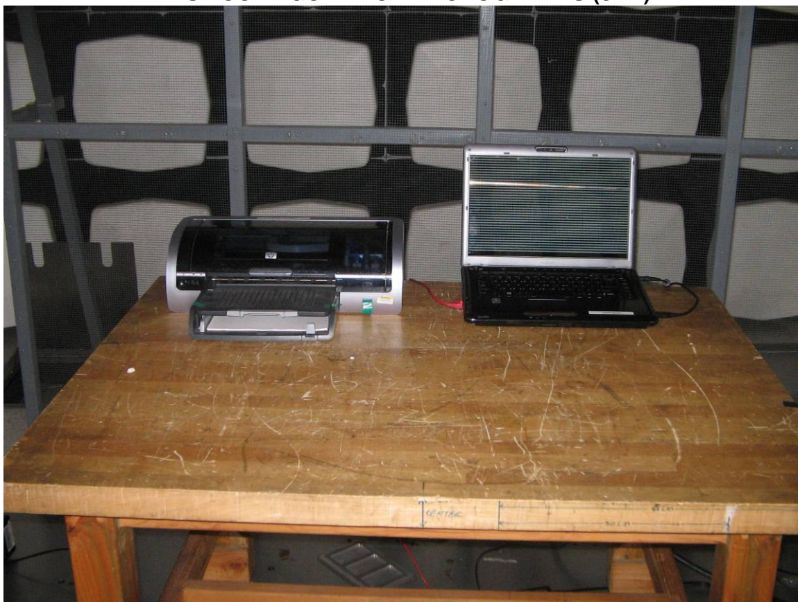
AC Power Port Conducted Emissions
