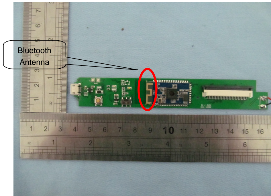
BACK VIEW OF PCB
