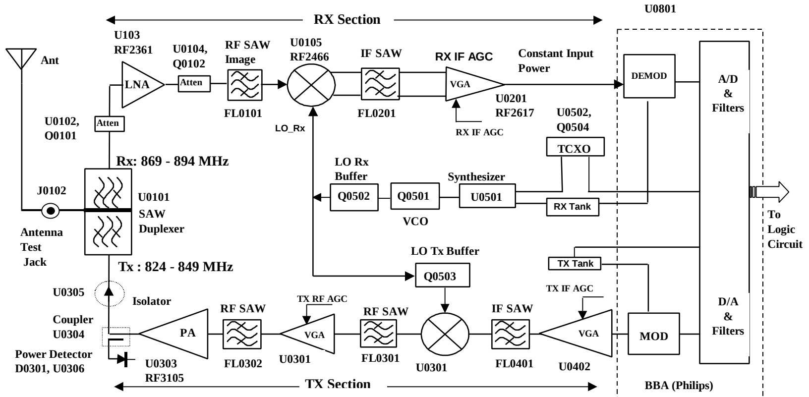
RF Block Diagram
