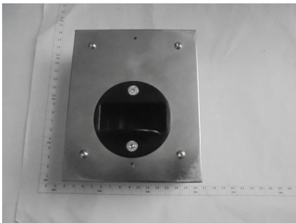
Photograph 1: EUT A Front side view
