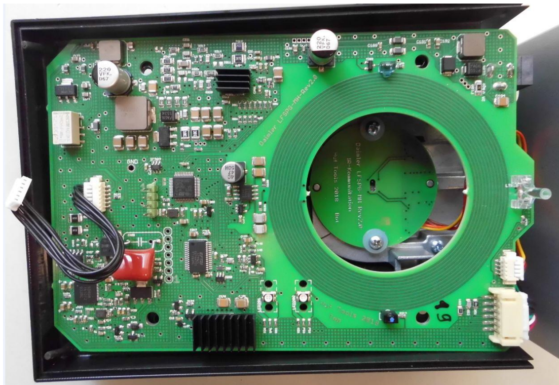
Photograph 1: EUT A – PCB top side
