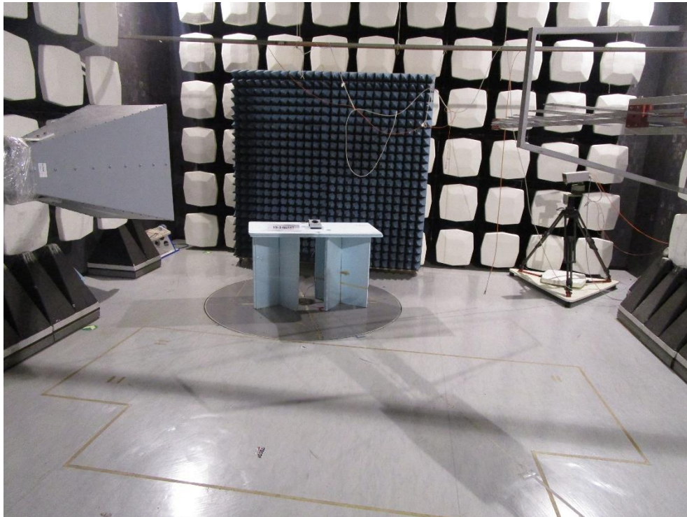
Photograph 3: overall view in the semi-anechoic chamber, EUT laying
