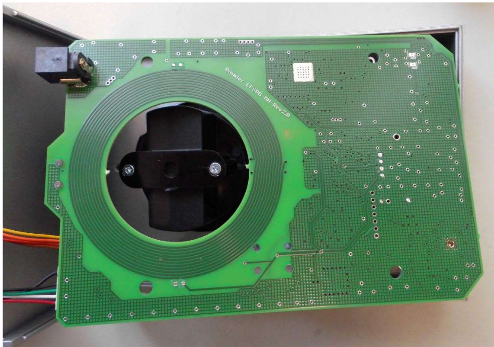
Photograph 2: EUT A – PCB rear side
