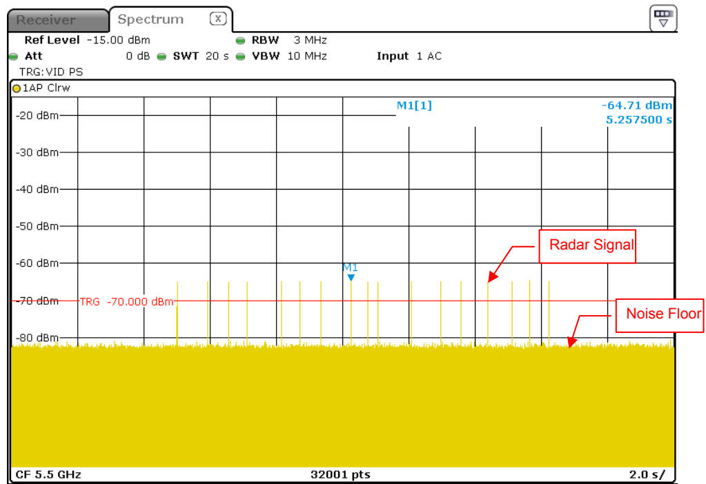
Radar Signal 5
